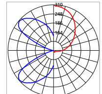
Max Candela linea 1ft 132.5° vertical = 306 180° horizontal = 306
